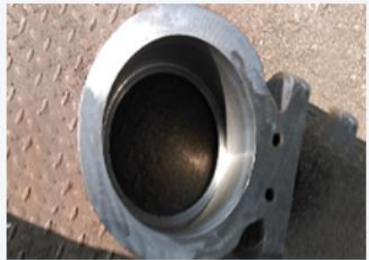
bearing housing for electrical loco DIN17182 material
